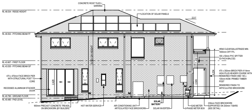
LEFT ELEVATION (WEST)
