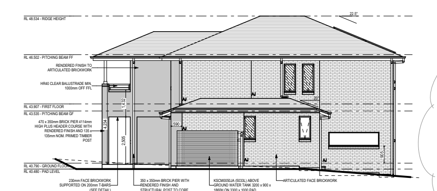
RIGHT ELEVATION (EAST)
